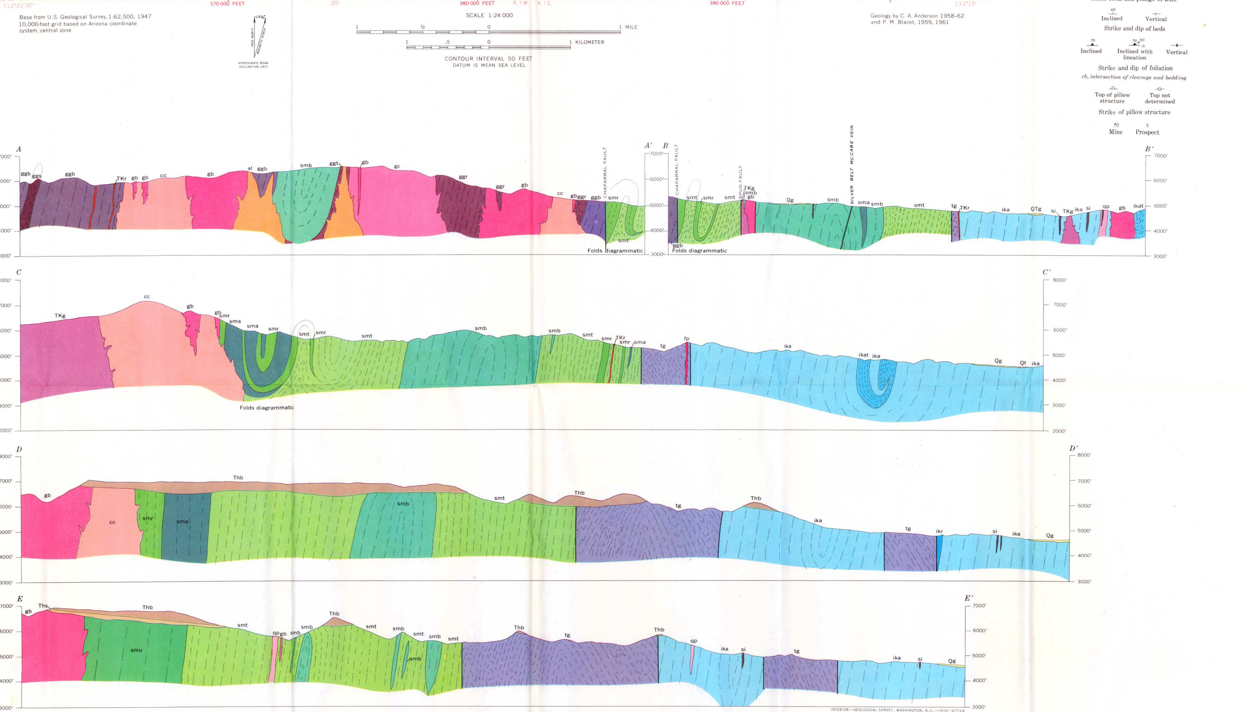
GEOLOGIC MAP OF THE NE 1/4 MOUNT UNION QUADRANGLE, YAVAPAI COUNTY, ARIZONA
