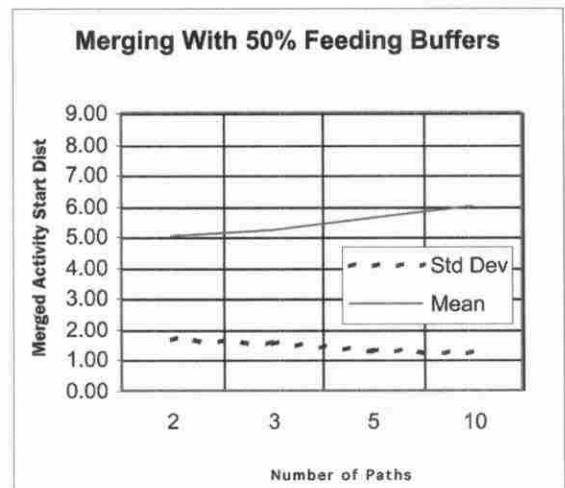
Figure 5. Feeding Buffers Mitigate Merge Bias
