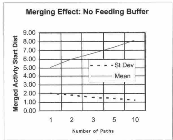
Figure 4. The Merging Effect Causes Late Bias
