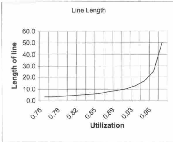
Figure 6. Queuing Causes Late Bias at Modest Resource Loading
