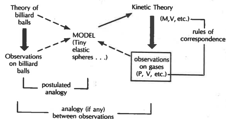
FIGURE 1.3 Observations, laws, theories, and models
