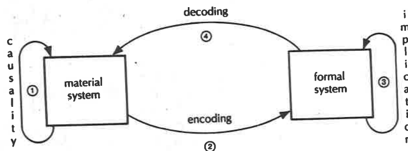
FIGURE 1.2 Newton's scheme for mathematical modeling
