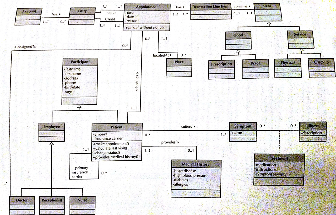
FIGURE 5-7 Sample Class Diagram
