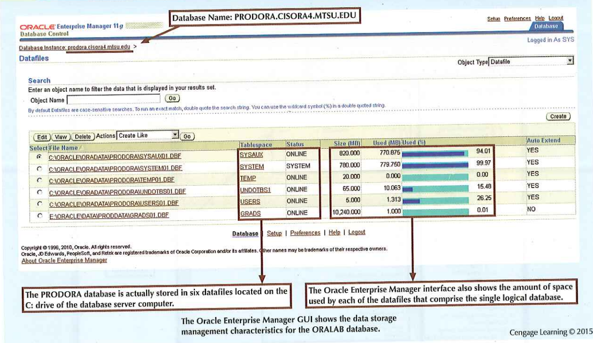
FIGURE 1.11 Illustrating data storage management with Oracle
