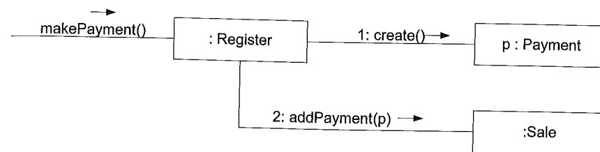
Figure 17.18 Register creates Payment.
