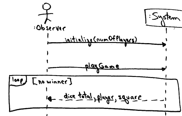
Figure 17.8 SSD for the Monopoly game. Note the playGame operation.
