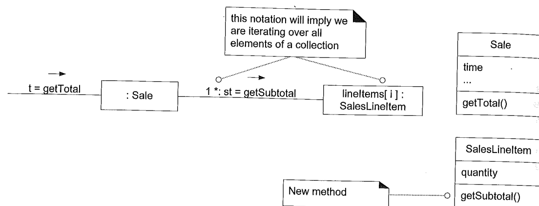
Figure 17.16 Calculating the Sale total.
