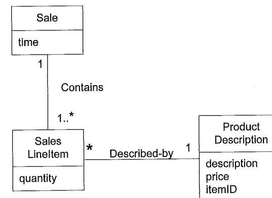
Figure 17.14 Associations of Sale.
