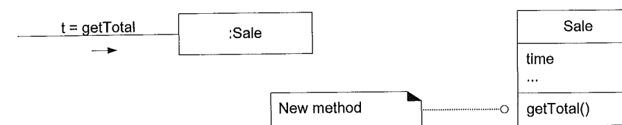
Figure 17.15 Partial interaction and class diagrams.
