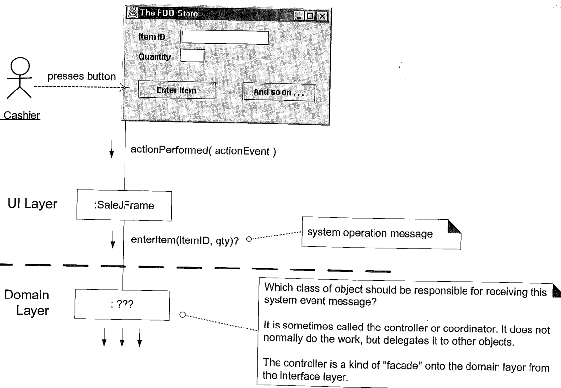
Figure 17.21 What object should be the Controller for enterItem?
