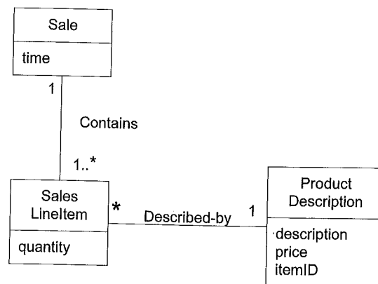
Figure 17.12 Partial domain model.
