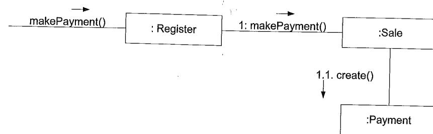
Figure 17.19 Sale creates Payment.
