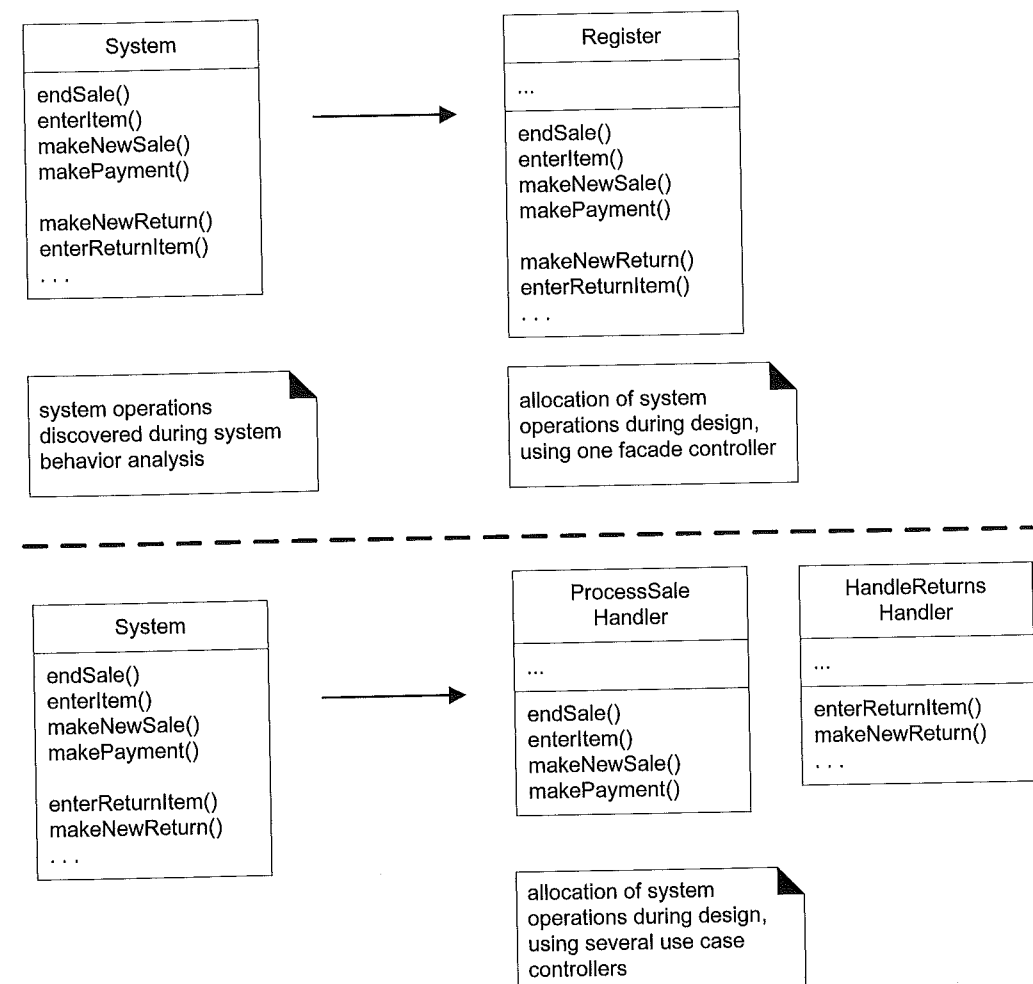
Figure 17.23 Allocation of system operations.
