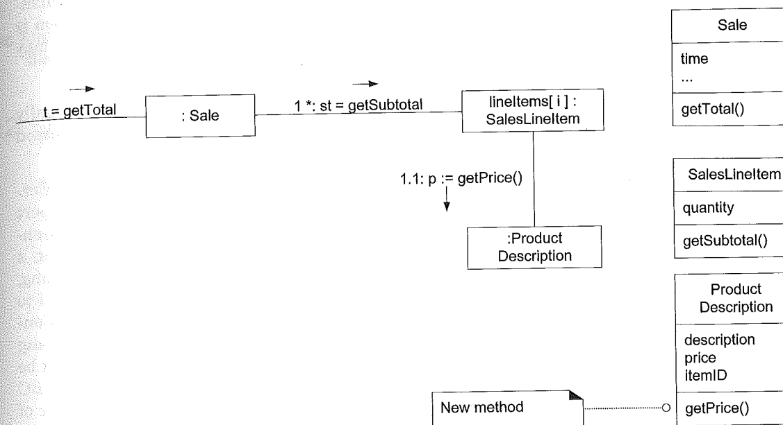
Figure 17.17 Calculating the Sale total.
