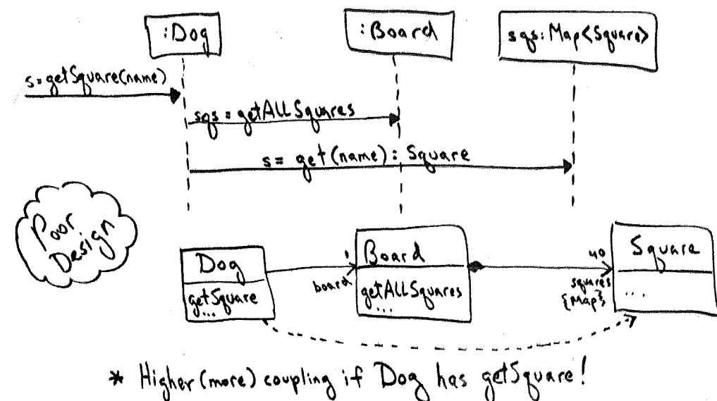
Figure 17.7 Evaluating the effect of coupling on this design.
