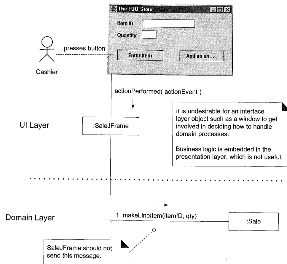
Figure 17.25 Less desirable coupling of interface layer to domain layer.
