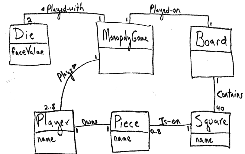
Figure 17.3 Monopoly iteration-1 domain model.
