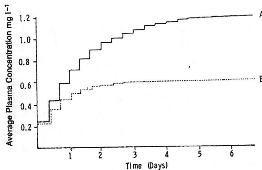
FIGURE 2.11 Accumulation of two compounds after multiple dosing. Compound A has a half-life of 24 hours, compound B of 12 hours. Dosing interval is 8 hours. From Timbrell, J. A., Principles of Biochemical Toxicology, Taylor & Francis, London, 2000.
