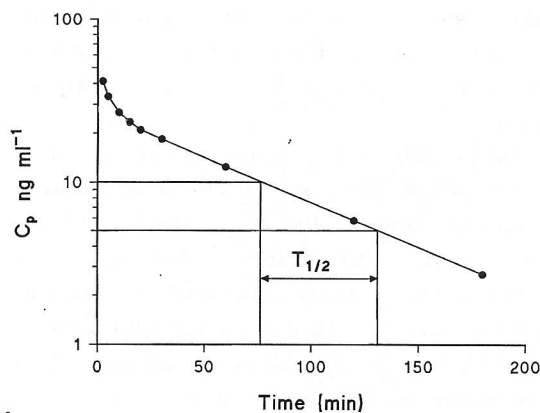
FIGURE 2.10 Plasma level of a chemical after intravenous administration. The plasma level is plotted on a log scale. The half life ( T_{1/2} ) can be determined as shown. The elimination rate constant ( k_{el} ) can be determined from the slope of the linear part of the line.
