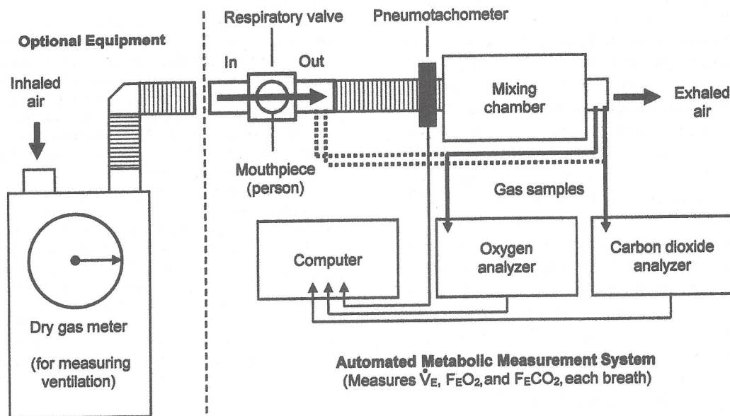
Figure 15.1 Schematic of the components of an automated (computerized) metabolic measurement system for measuring ventilation ( \dot{V}_E ) and the fractions of exhaled \text{O}_2 ( F_{E\text{O}_2} ) and \text{CO}_2 ( F_{E\text{CO}_2} ). In some cases, gas samples are drawn from the respiratory valve (instead of the mixing chamber) and \dot{V}_E is measured with a turbine or spirometer (usually if nonautomated). Optionally, a dry gas meter can be used to measure inhaled (or exhaled) ventilation.
