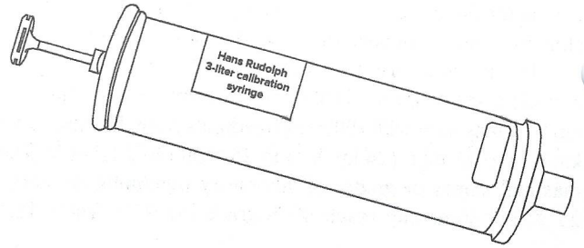
Figure 15.3 A 3-liter calibration syringe is used to calibrate the exhaled volume measured by the flow volume meter (pneumotachometer).
