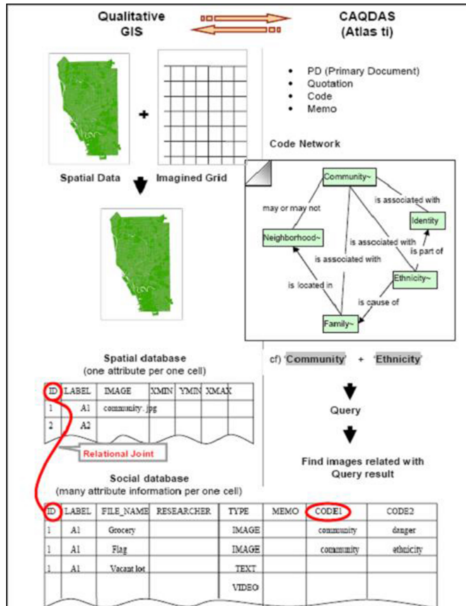
Figure 3: Jin-Kyu JUNG's "CAQ-GIS" program [35]
