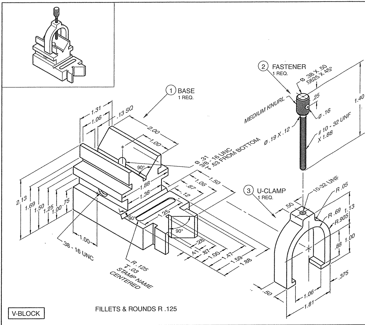
Figure 11.68 V-block
