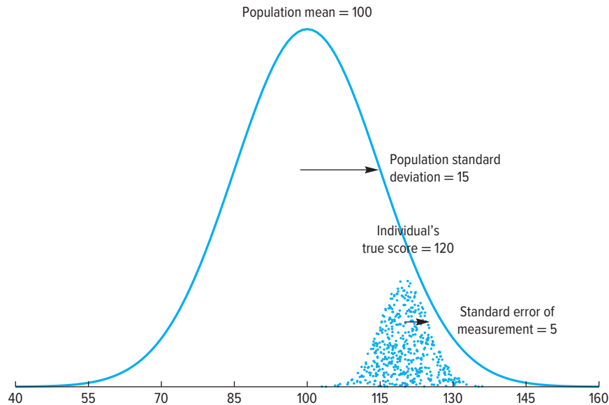
Figure 5–1 Possible observed scores for an individual with a true score of 120.
