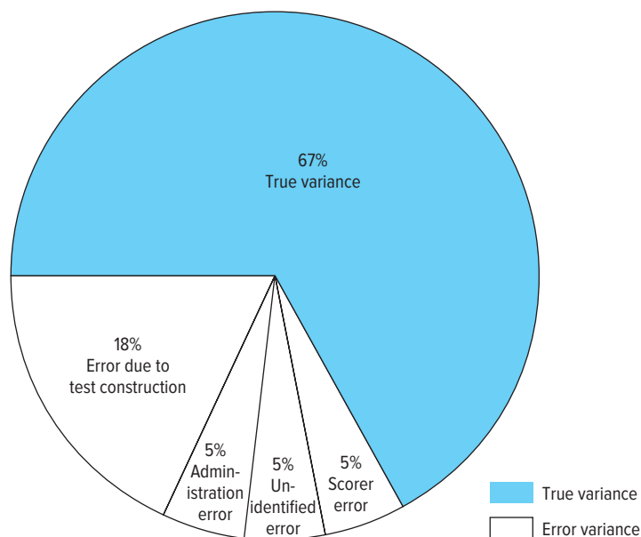
Figure 5–5 Sources of variance in a hypothetical test.
