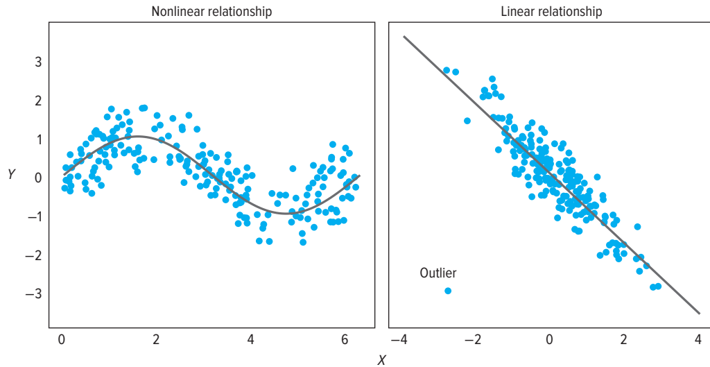
Figure 3-17 Scatterplot showing nonlinear and linear relationships.
