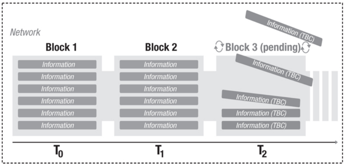
Figure 1 Blockchain infrastructure
