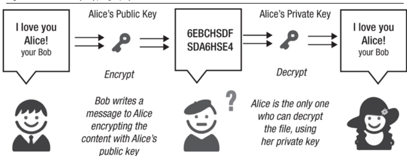
Figure 3 Public-key cryptography
