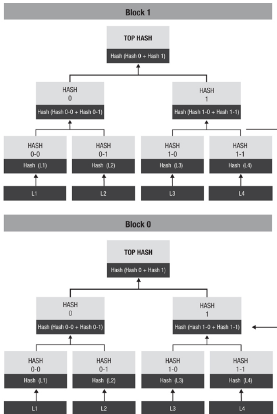
Figure 5 A schematic representation of a blockchain
