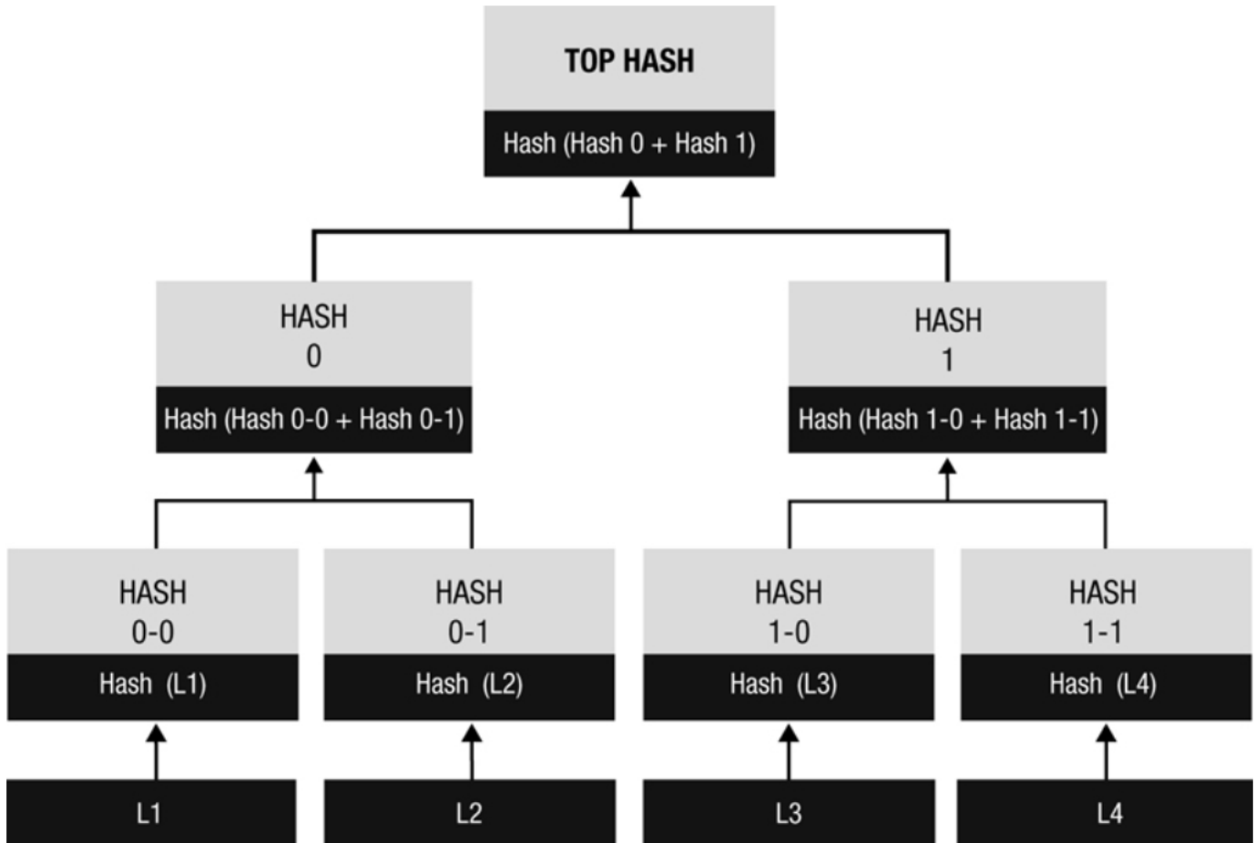
Figure 4 A Merkle tree
