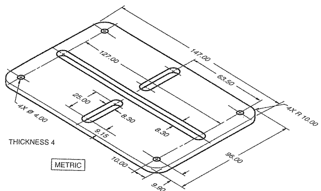
Figure 5.152 Offset plate
