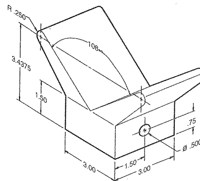
Figure 5.129 Snubber
