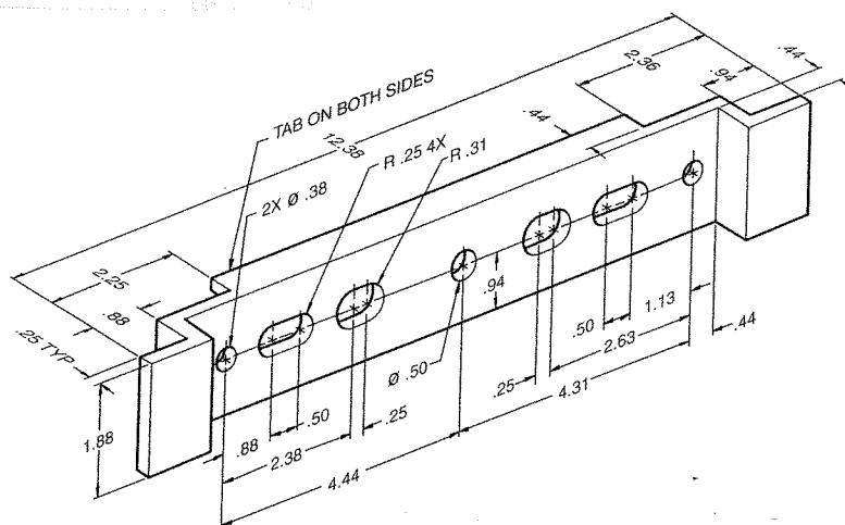
Figure 5.133 Control back
