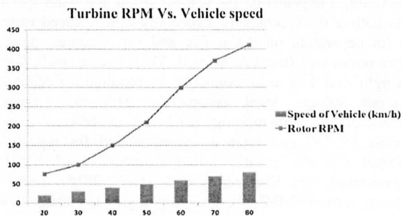
Figure-6. Turbine RPM Vs. Vehicle speed.
