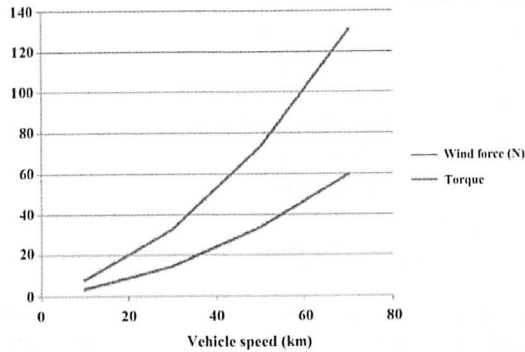
Figure-7. Vehicle speed vs. produced torque and wind force.
