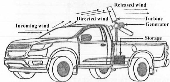
Figure-1. The VMWT system.
