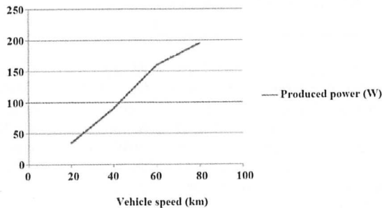
Figure-8. Produced power (w) vs. vehicle speed.
