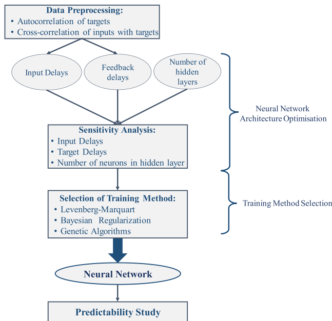
Fig. 1. Framework for tuning NARX neural network parameters and selecting the training method.
