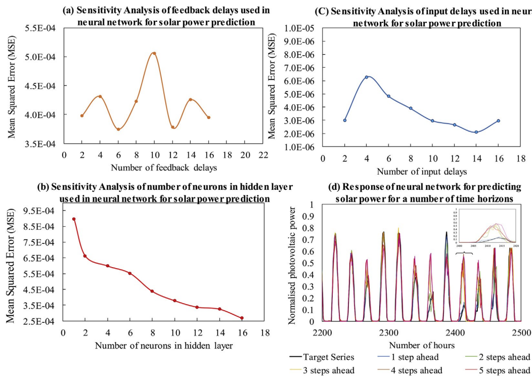
Fig. 7. The sensitivity analysis and performance of ANN for solar power prediction.
