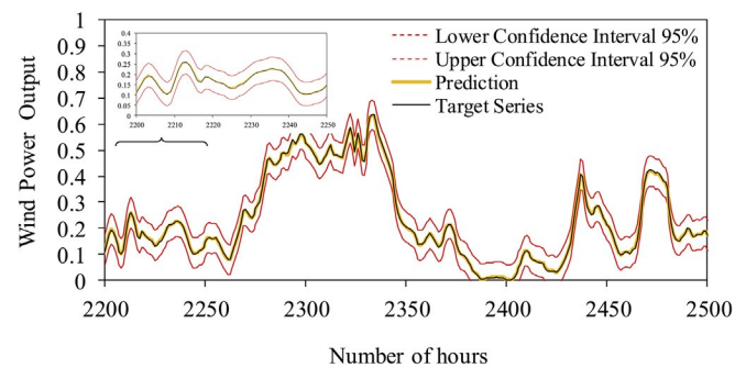
Fig. 5. Time series response of GPR for wind power prediction (present time) magnified for observation purposes.
