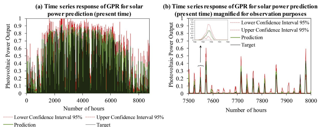
Fig. 9. (a) Time series response of GPR for solar power prediction (present time) and (b) Time series response of GPR for solar power prediction (present time) magnified for observation.
