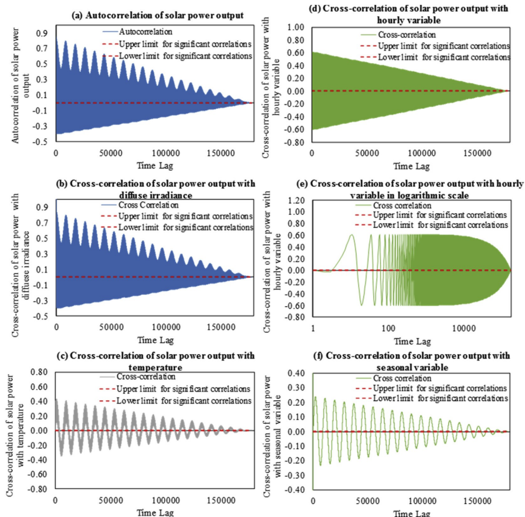
Fig. 6. Cross-correlations for input data applied for the solar power prediction.
