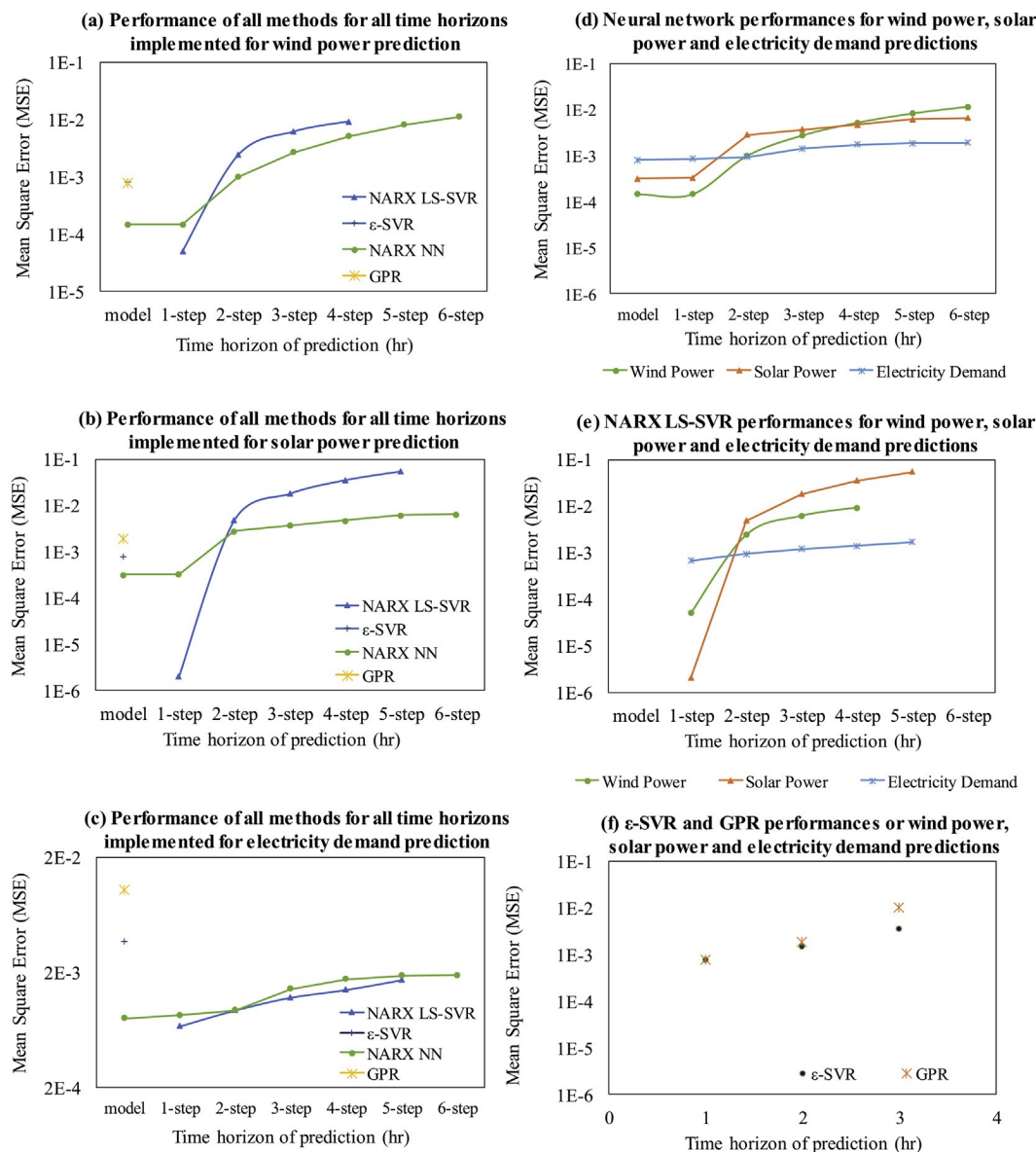
Fig. 15. Comparison of the prediction methods for wind and solar power as well as demand.
