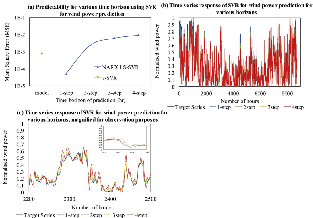
Fig. 4. The sensitivity analysis and performance of the SVR for wind power prediction.
