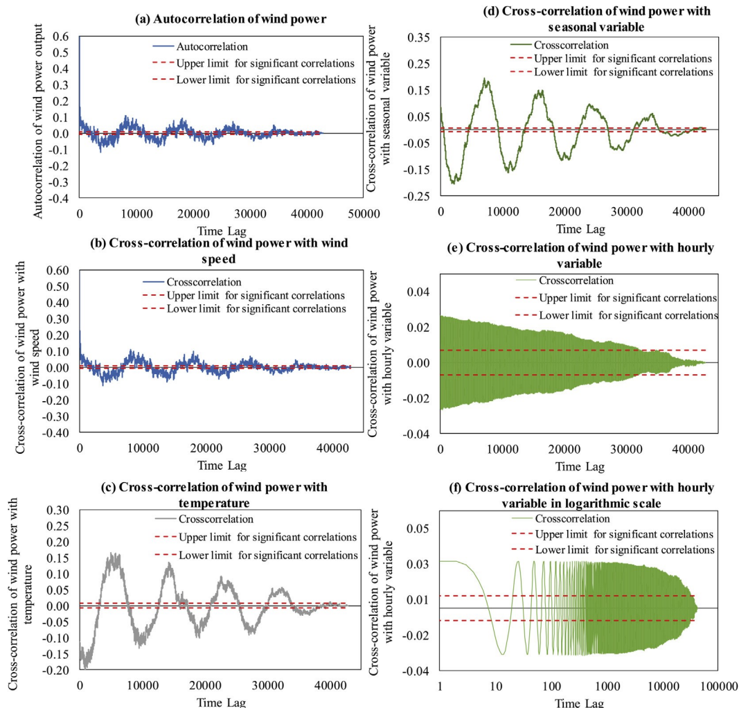
Fig. 2. Cross-correlations for input data applied for the wind power prediction.
