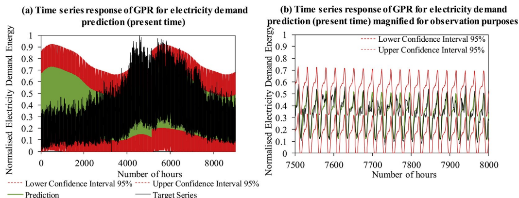
Fig. 14. (a) Time series response of GPR for electricity demand prediction (present time), (b) Time series response of GPR for electricity demand prediction (present time) magnified for observation purposes.
