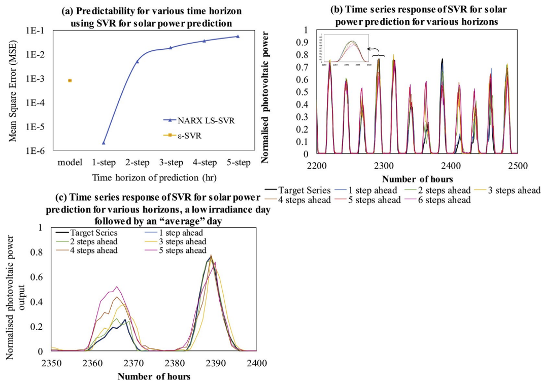
Fig. 8. The sensitivity analysis and performance of SVR for solar power prediction.
