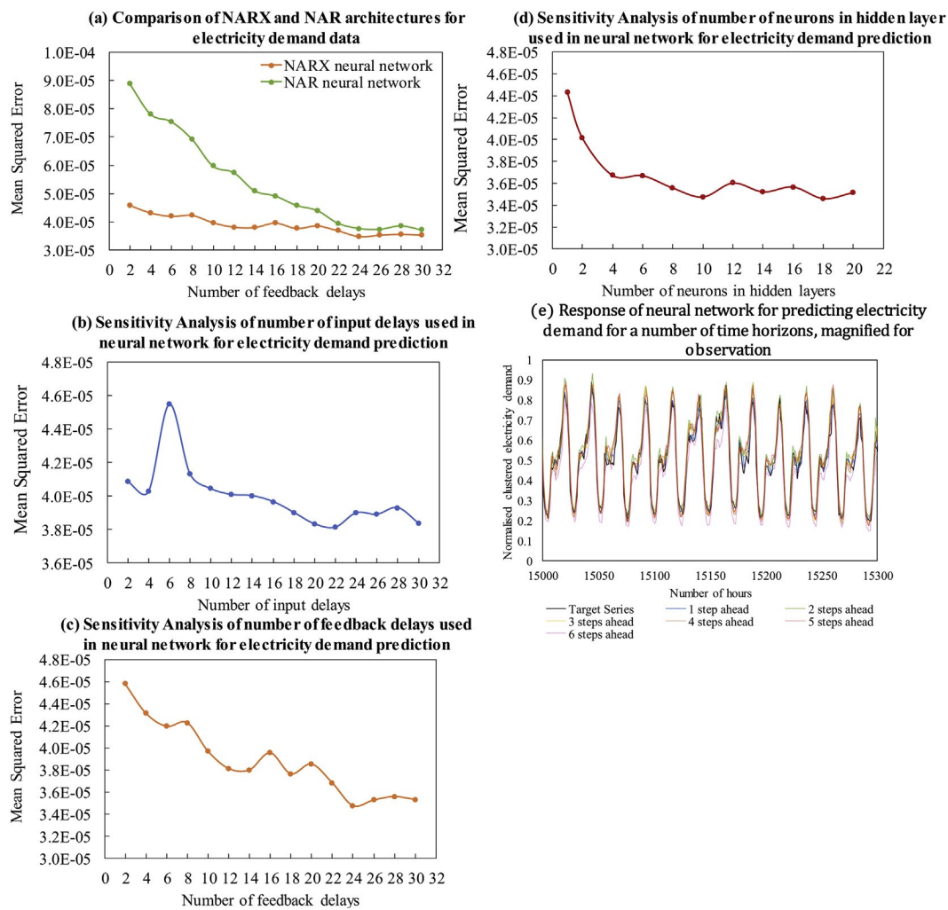
Fig. 12. The sensitivity analysis and performance of ANN for electricity demand prediction.
