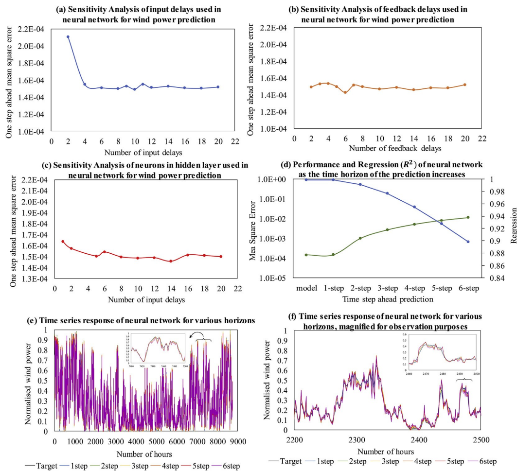
Fig. 3. The sensitivity analysis and performance of ANN for wind power prediction.
