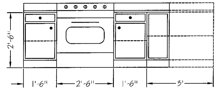
KITCHEN
