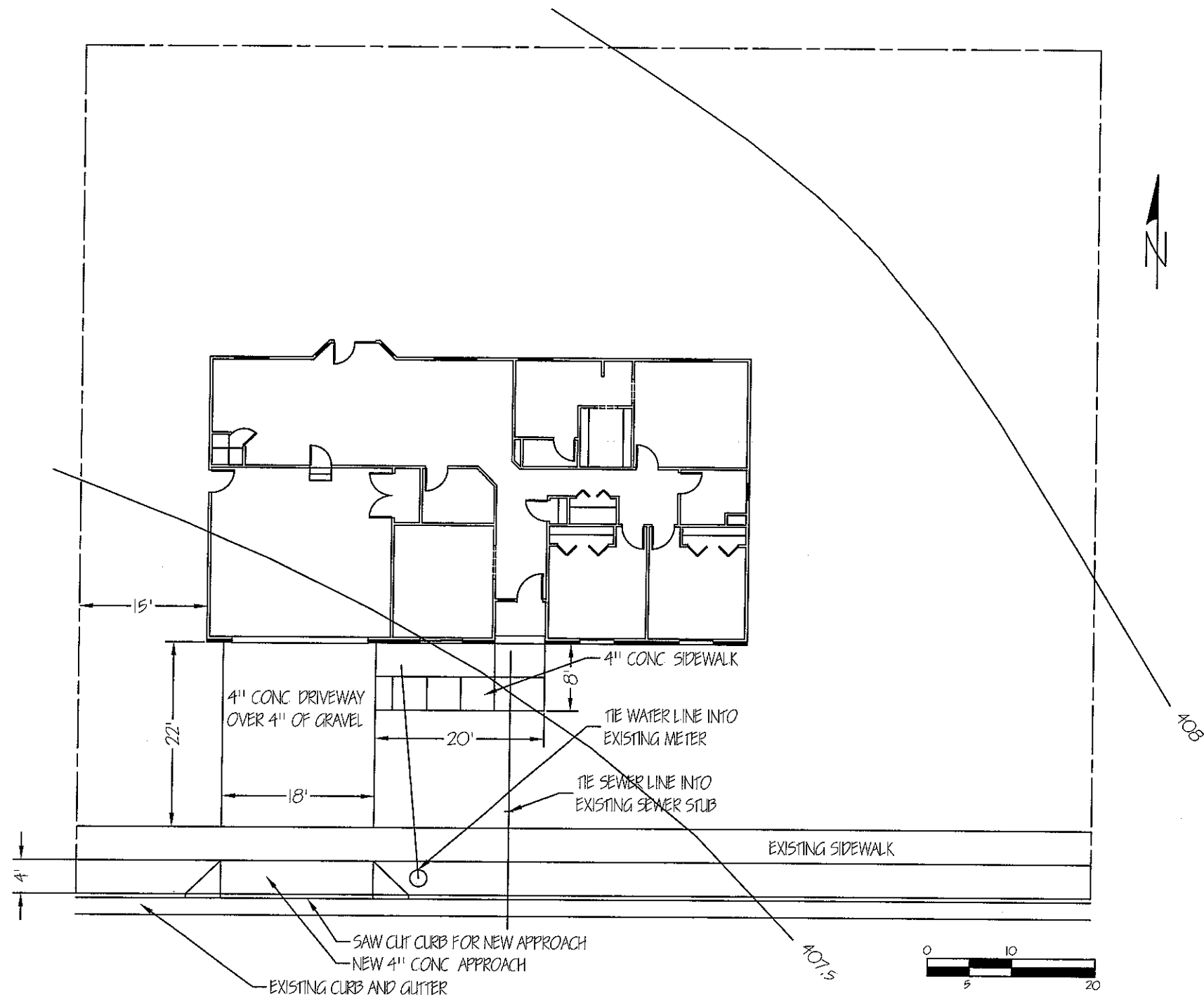
SITE PLAN
