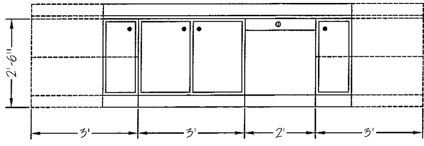
KITCHEN
