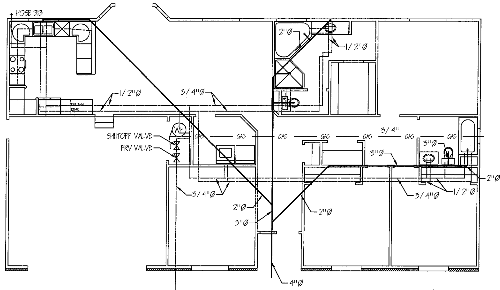
FLOOR PLAN
