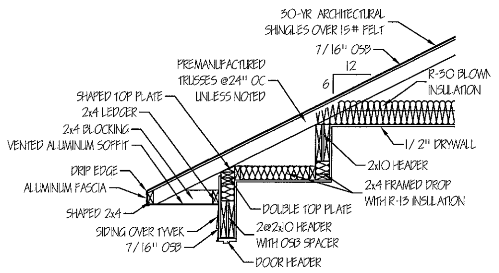
10 A8 EAVES SECTION
