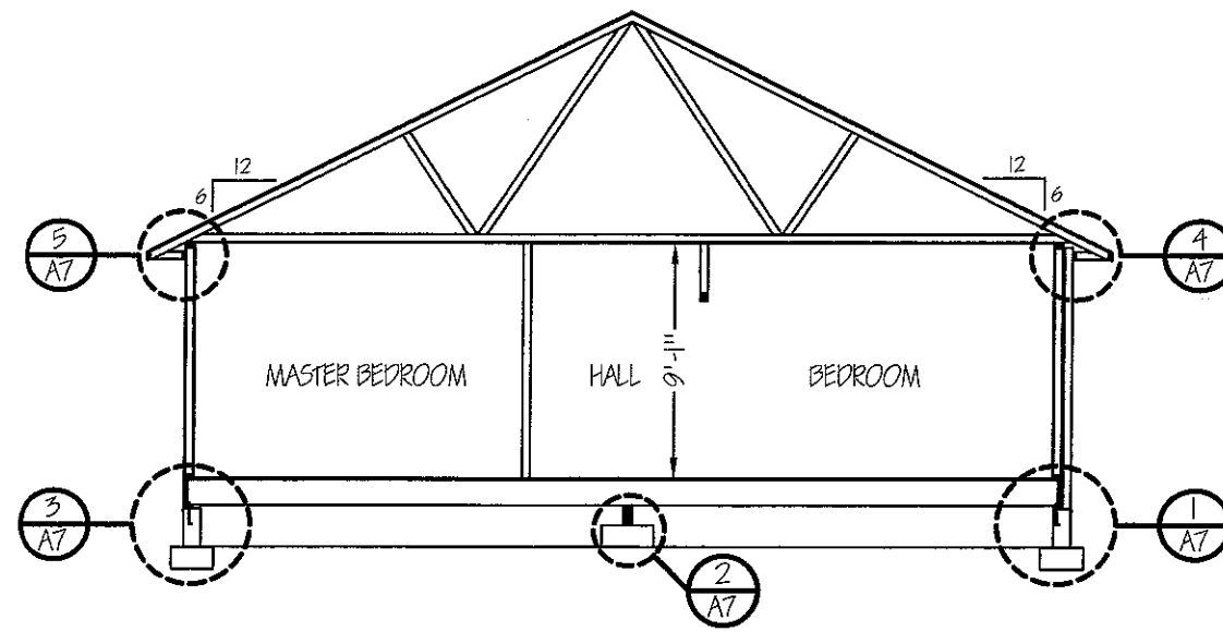
A BUILDING SECTION A5
