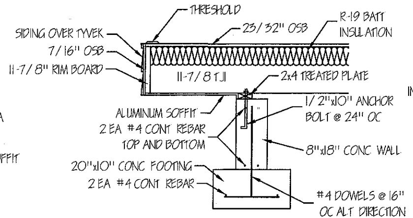
8 A8 FOOTING SECTION
