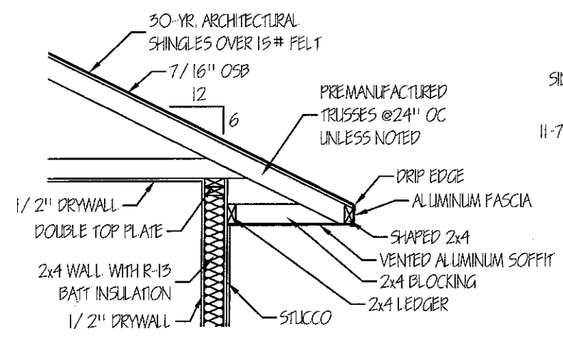
9 A8 EAVES SECTION
