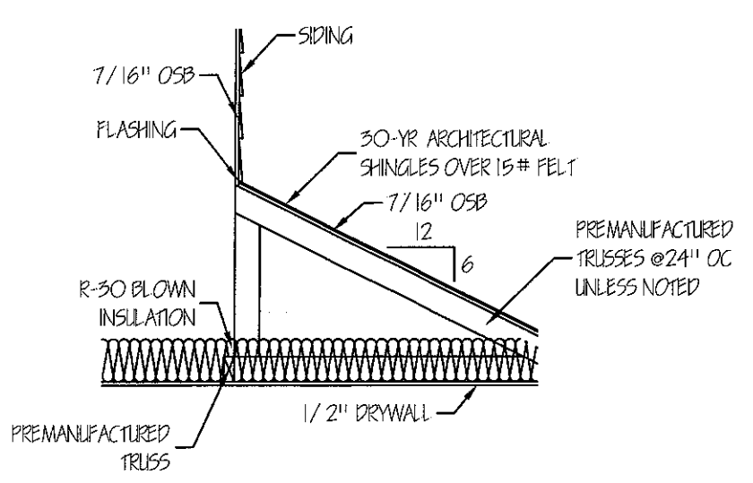
11 A8 EAVES SECTION
