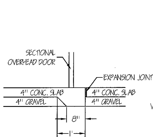
6 SLAB SECTION A7
