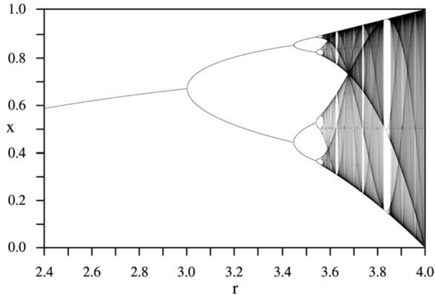
Fig. 4.2 Bifurcation diagram. (Source: Wikipedia)
