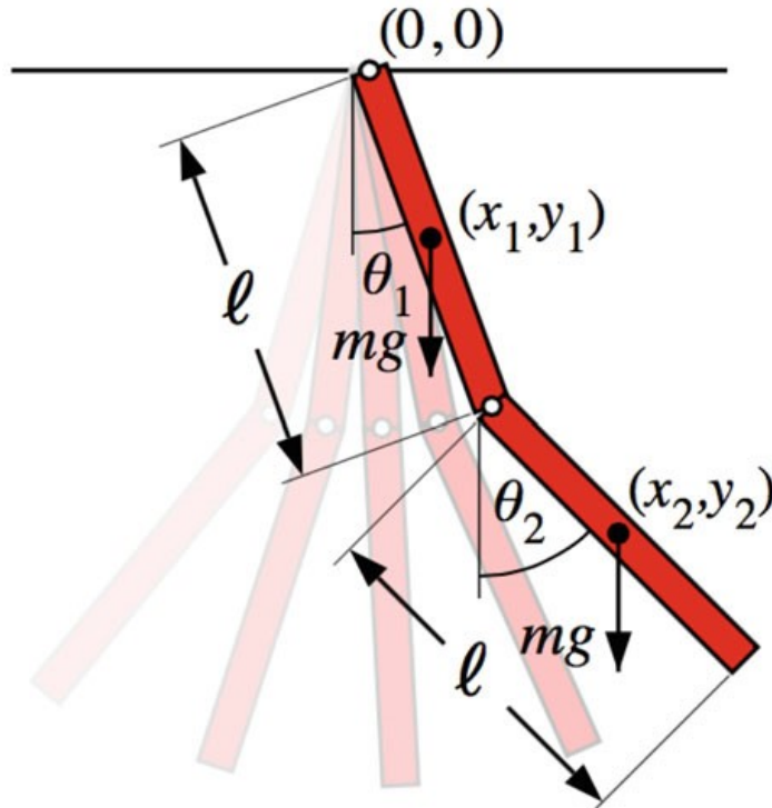
Fig. 4.1 Double pendulum. (Source: Wikipedia)
