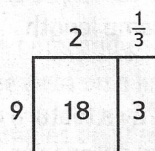
Area model for 2\frac{1}{3} * 9
