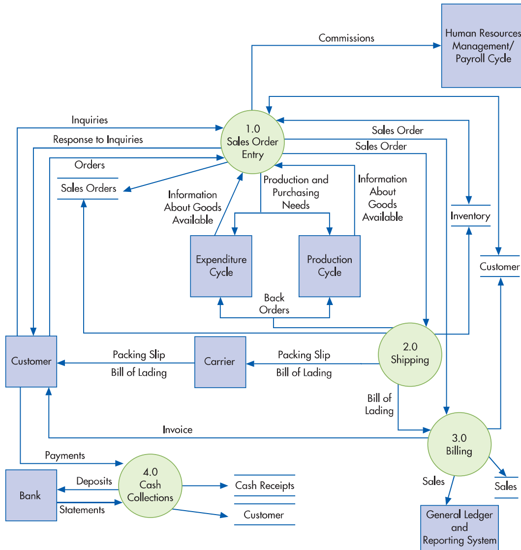
FIGURE 12-3 Level 0 Data Flow Diagram: Revenue Cycle
