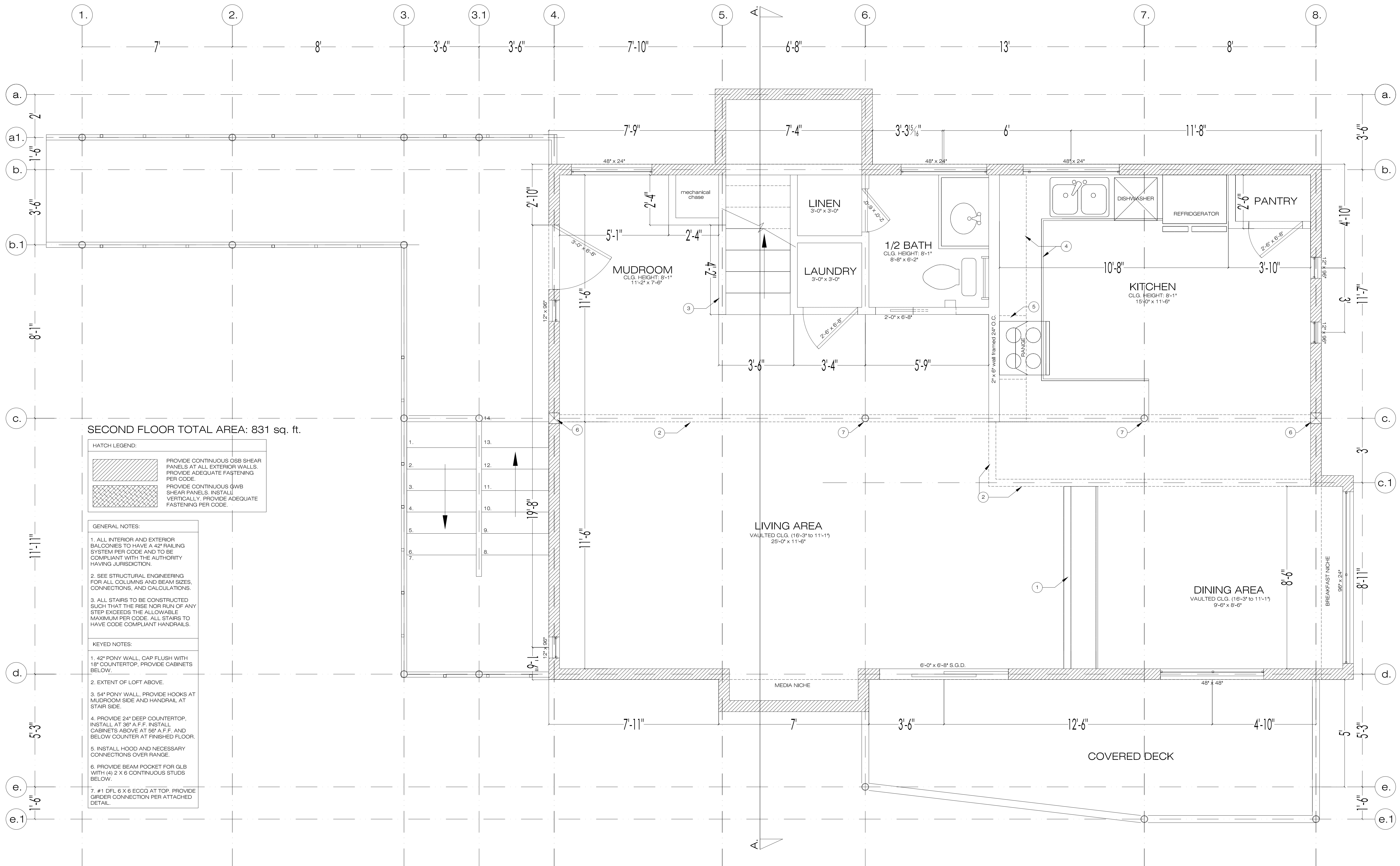
SECOND FLOOR PLAN SCALE: 1/2" = 1' NORTH
